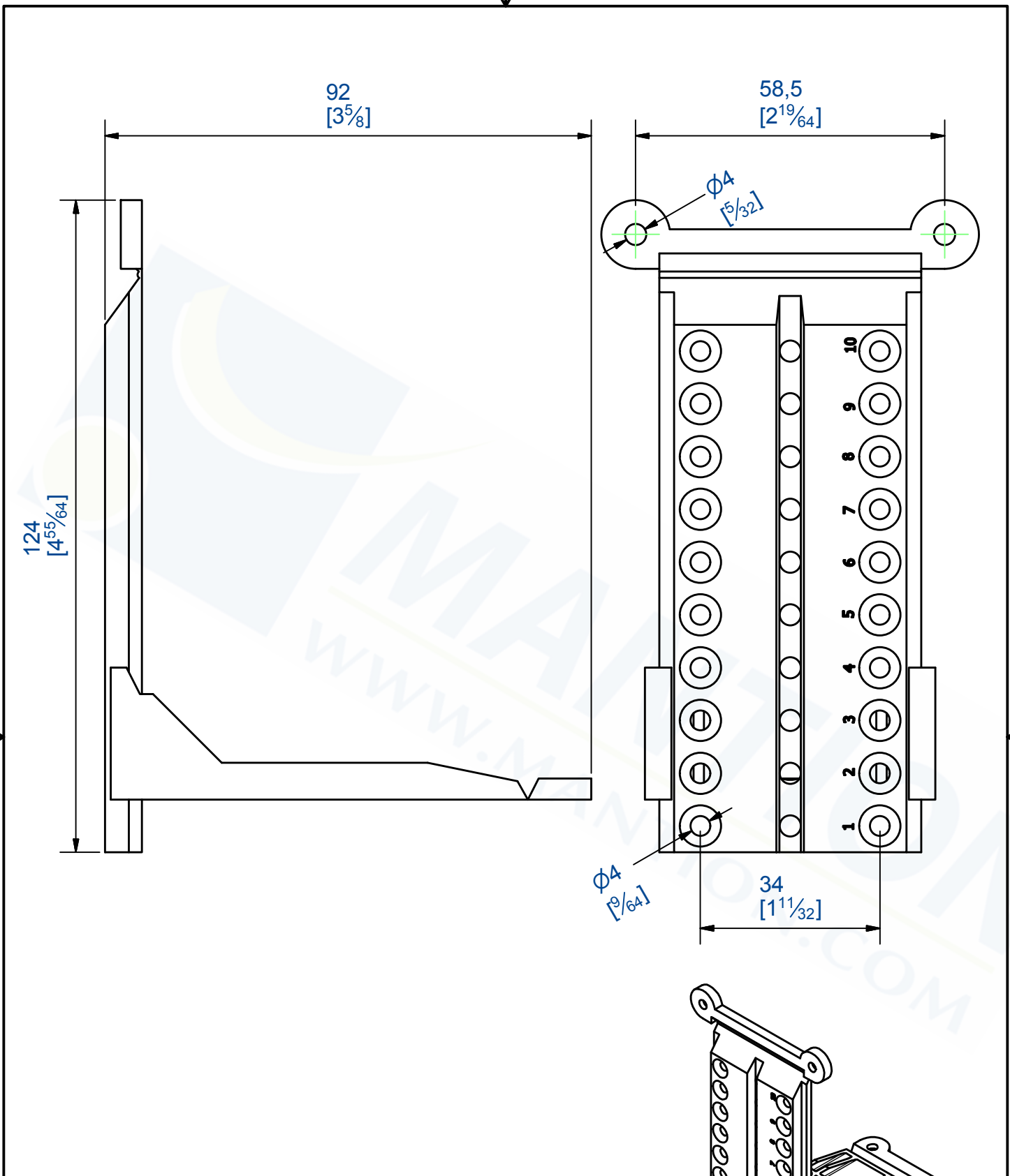
Kit de fixation sous pente Mounting kit for slanted ceiling
