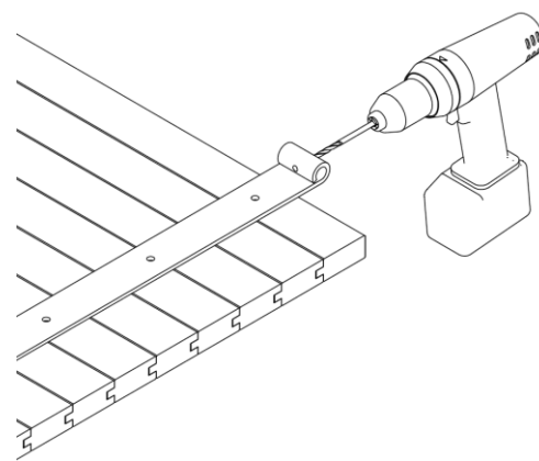
Parallel drilling
