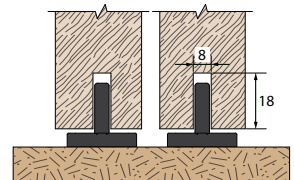
Montage 1103R + rainure
