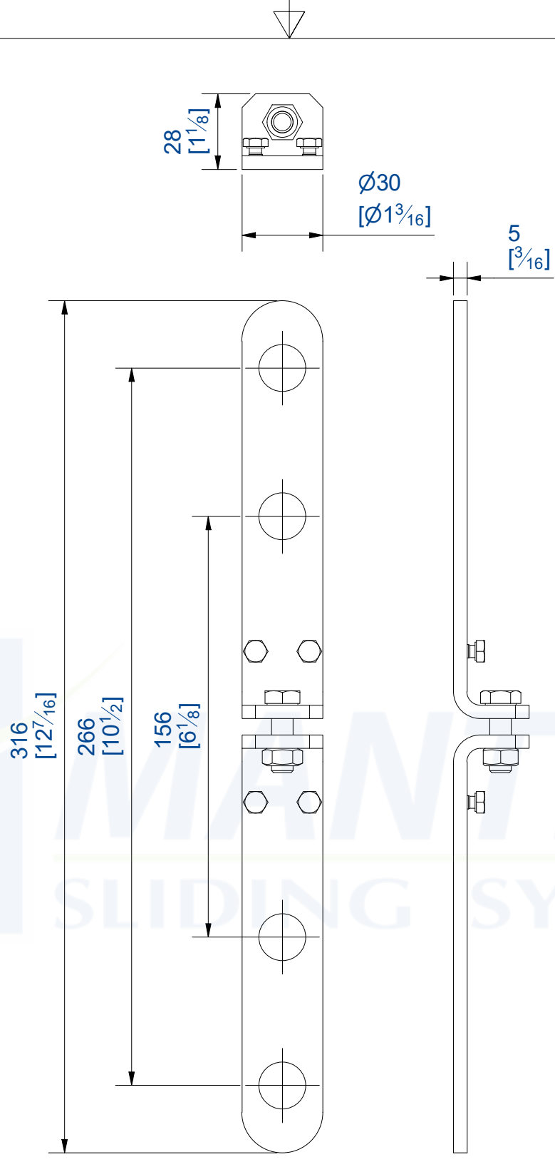
Kit de raccordement de rails ROCDESIGN noir Black connector for ROCDESIGN tracks
