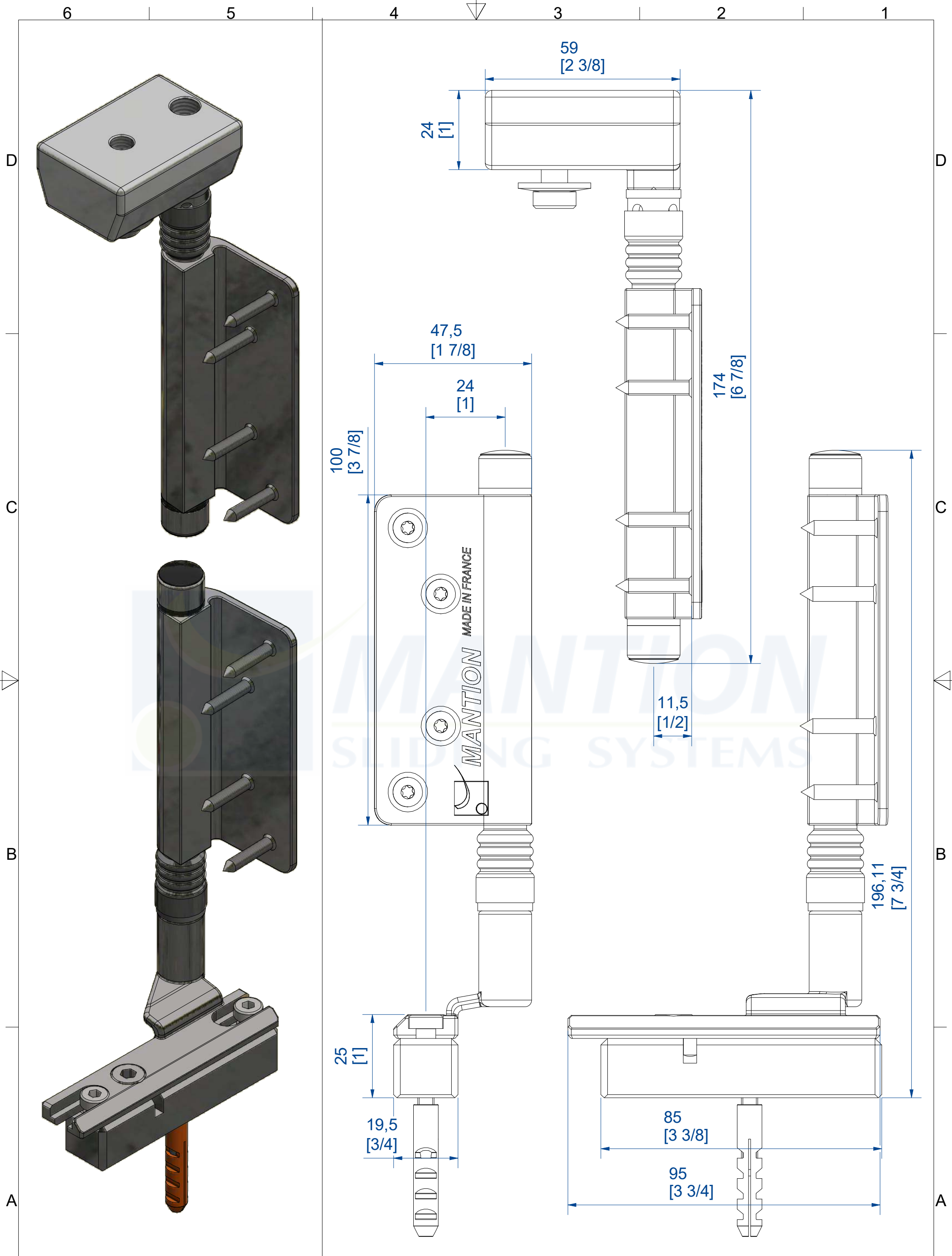
Set point fixe droit FWF100 Set right pivot assembly FWF100
