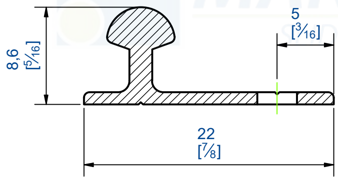
A-A (Ech. 3/1 )
