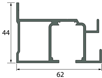
Rail SAF®-BOIS (1.85 m)
