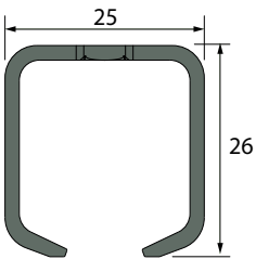
Rail 2526F - ALUMINIUM
