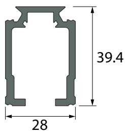
Rail SAF® 120 (13312) (3 - 6 m)
