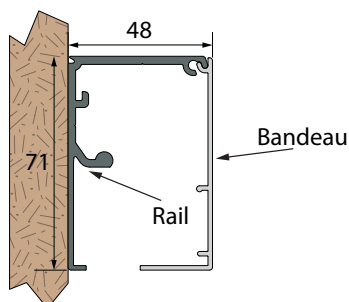
Rail fixation murale + bandeau
