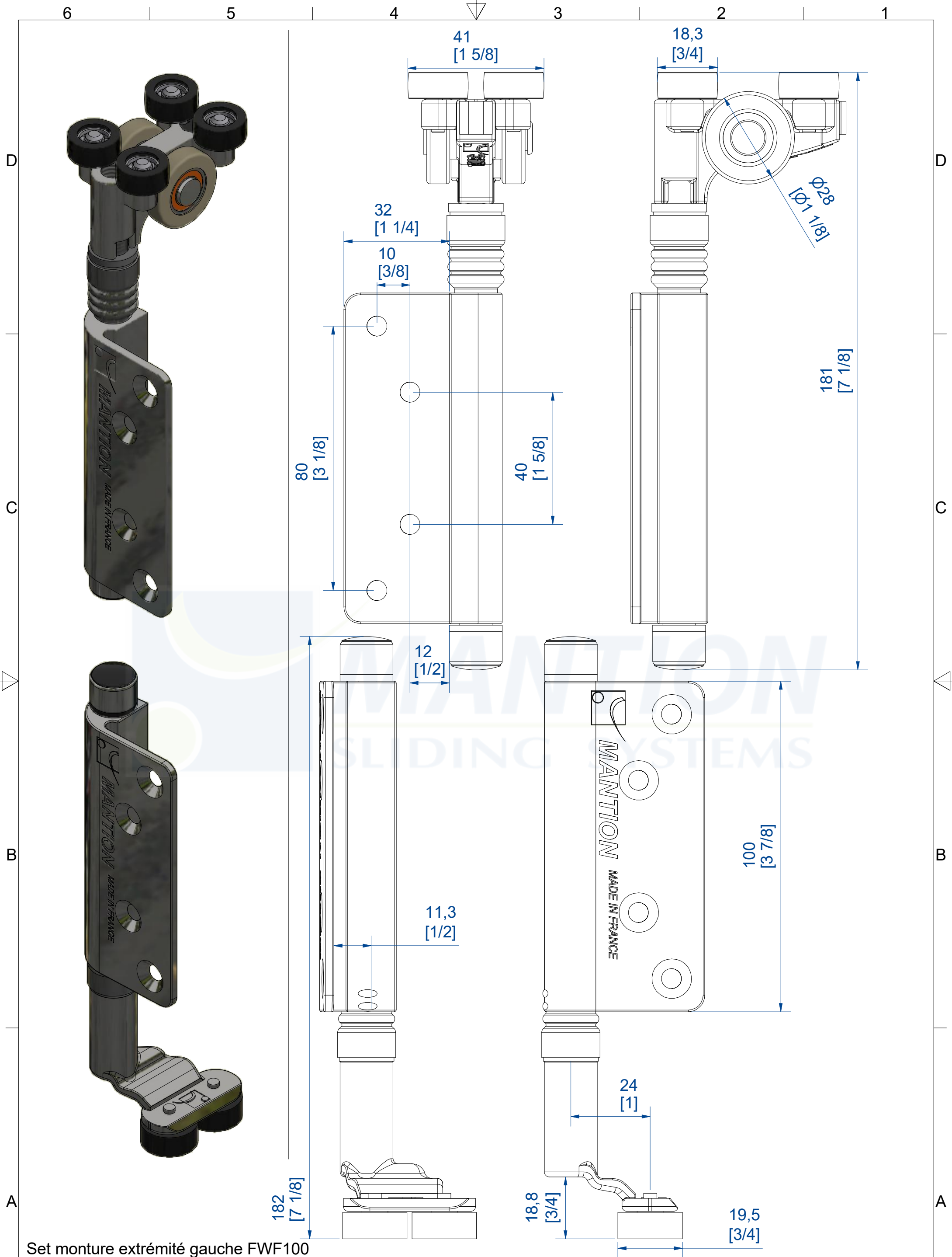
Set left end hanger FWF100
